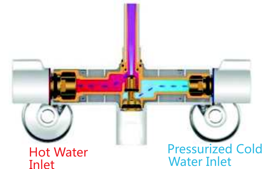
Mixing Water Outlet
